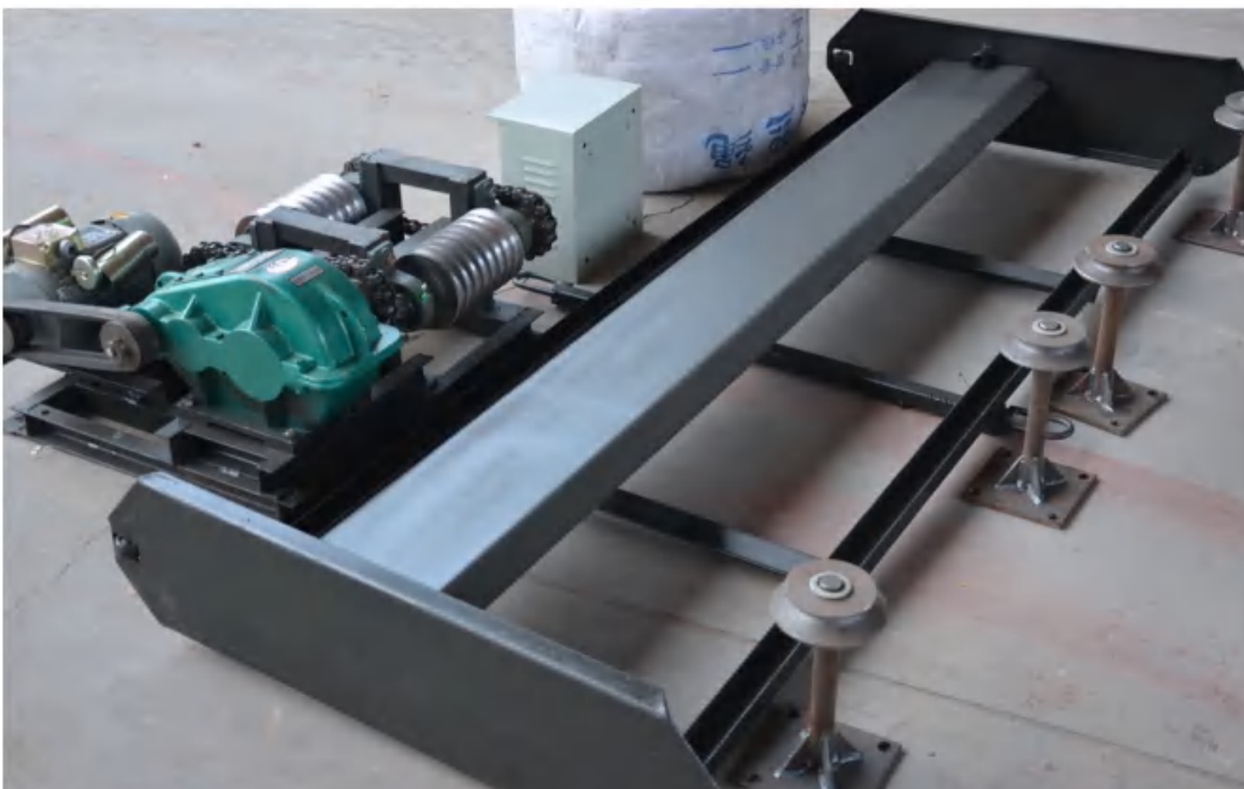
horizontal & slant manure cleaning belt
