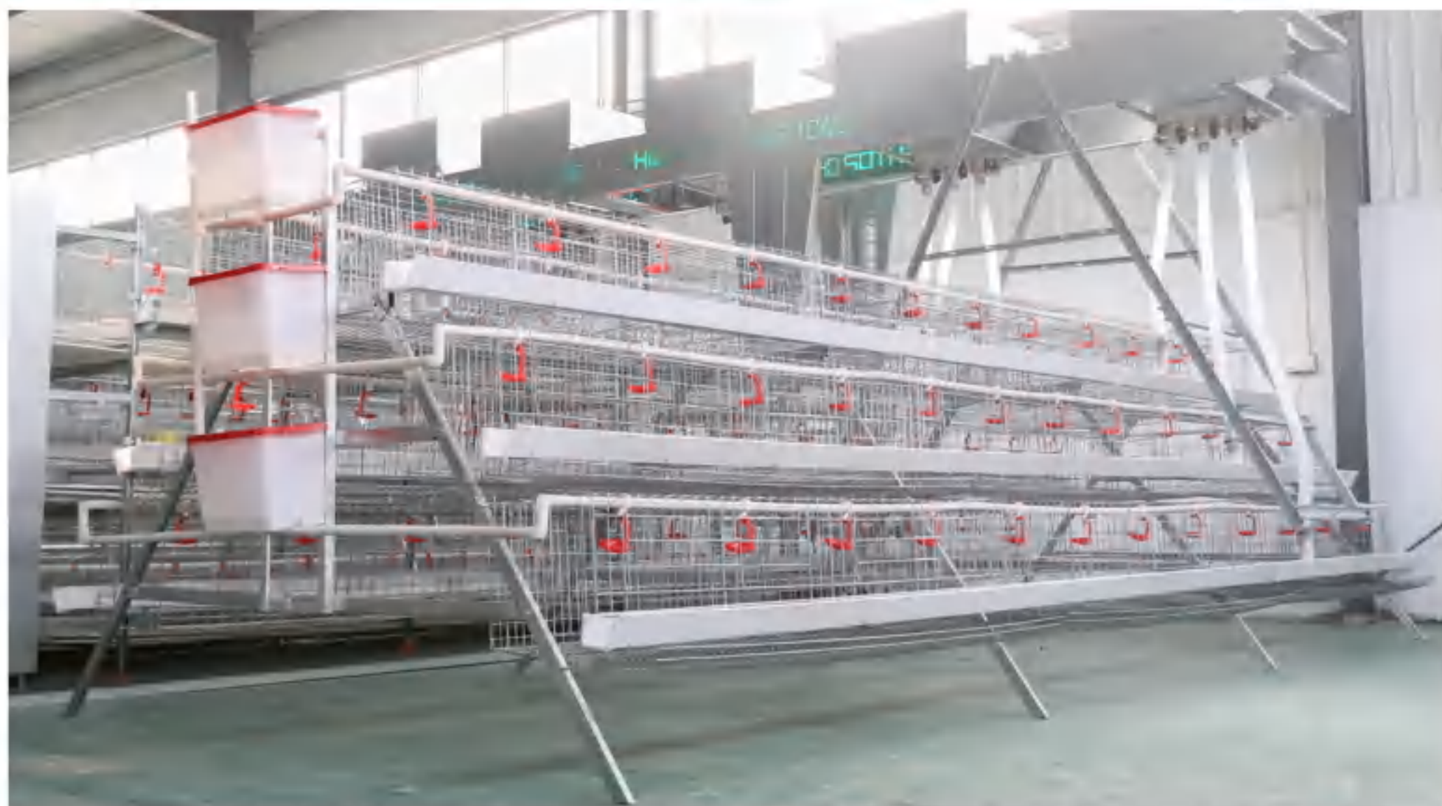
The specifications of layer cage ("HT" – Hightop® brand; "A" – A shape; "34" – 3 tiers 4 nests/doors; "L" – Large size)
