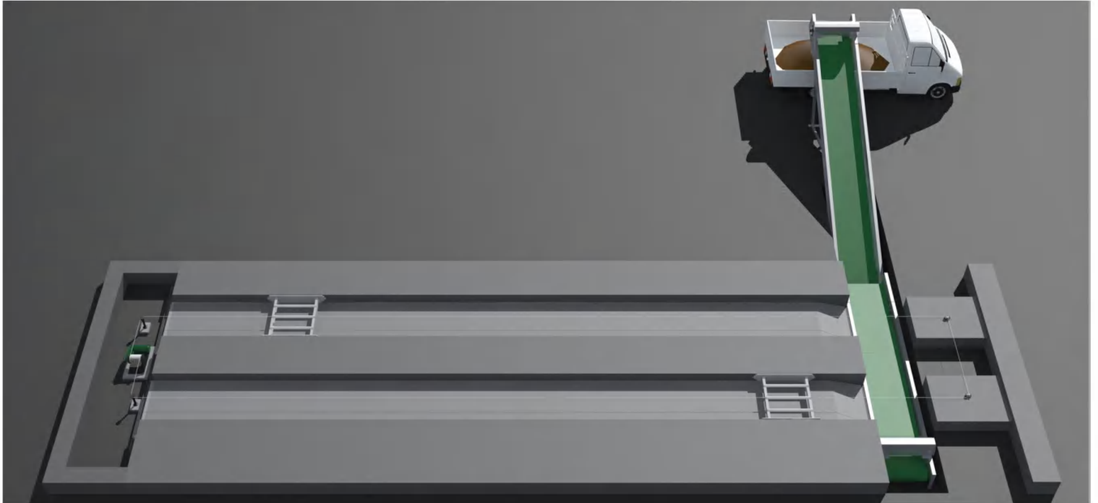
Scraper type automatic manure cleaning machine
